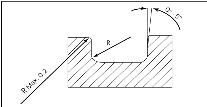
Figure 31 Groove specifications
