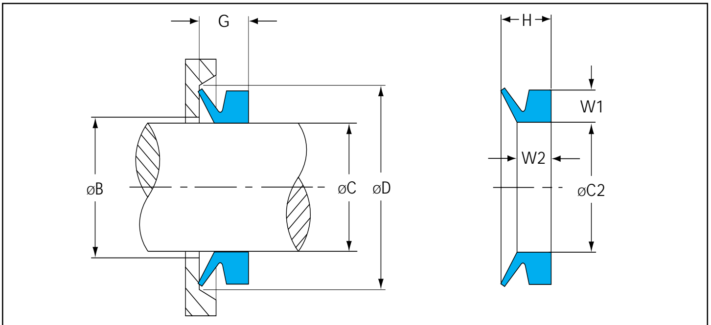
Figure 18 Installation drawing
