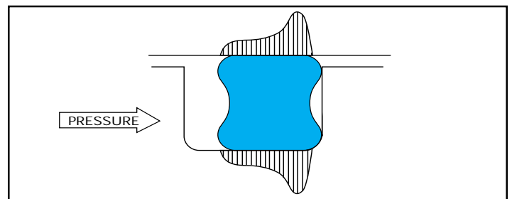
Figure 19 QUAD-RING® Seal load distribution profile
