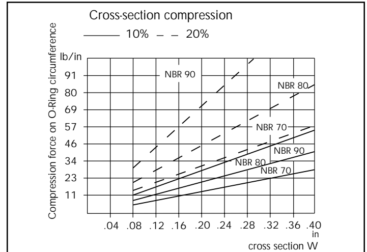
Figure 28 Compression forces on the O-Ring circumference depending on the Compound.
