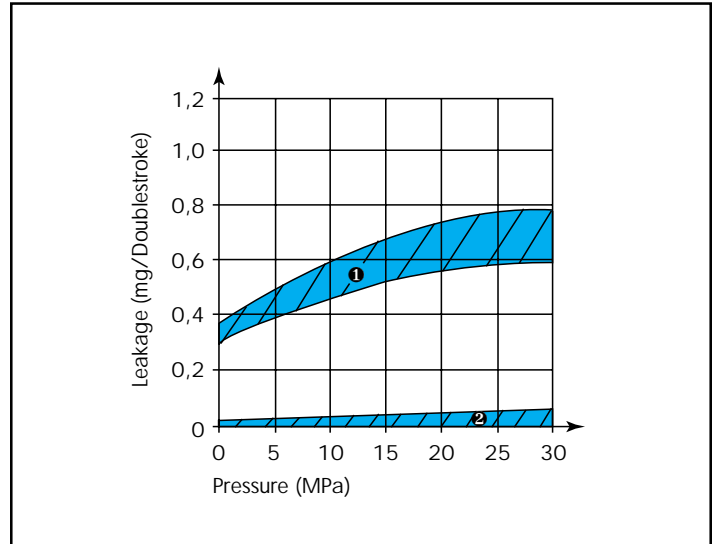
Figure 6 1) O-Ring with two Back-up rings 2) Turcon® Stepseal® K
